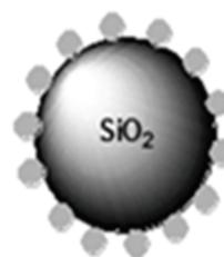
N-N-Dimethyl-N-Octadecyl-3-aminopropyl
